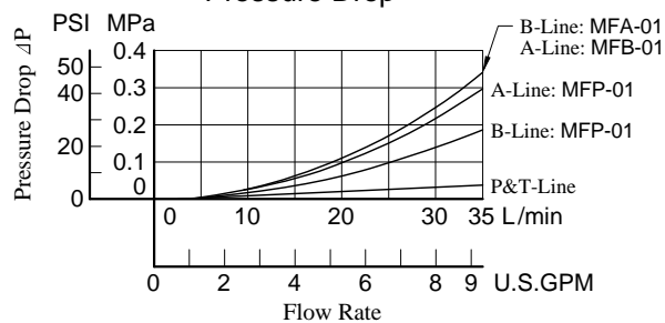
Pressure Drop
