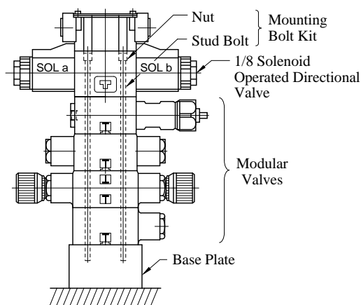
01 Series Modular Valve Assembly
